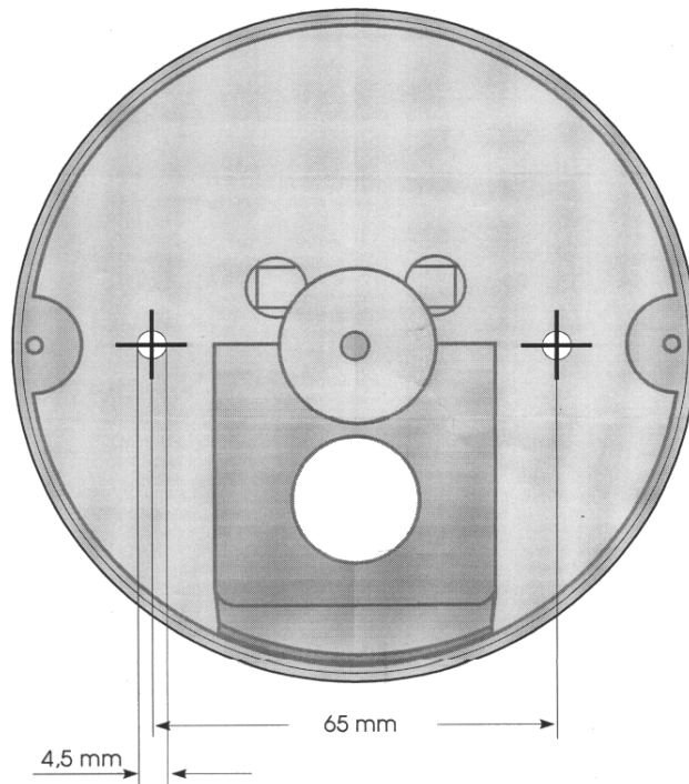
Fig.4: mounting of the bottom part
