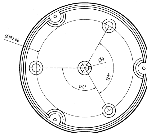
cable entry and mounting holes
