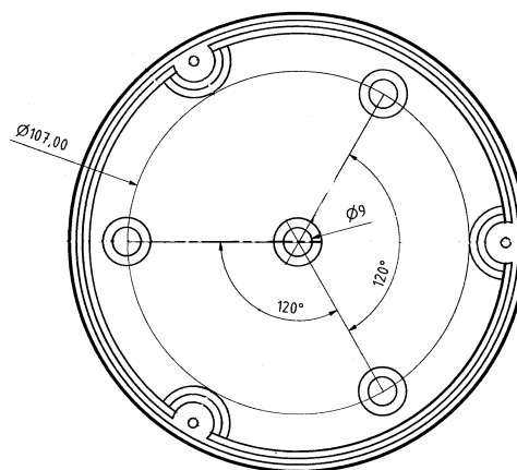
cable entry and mounting holes
