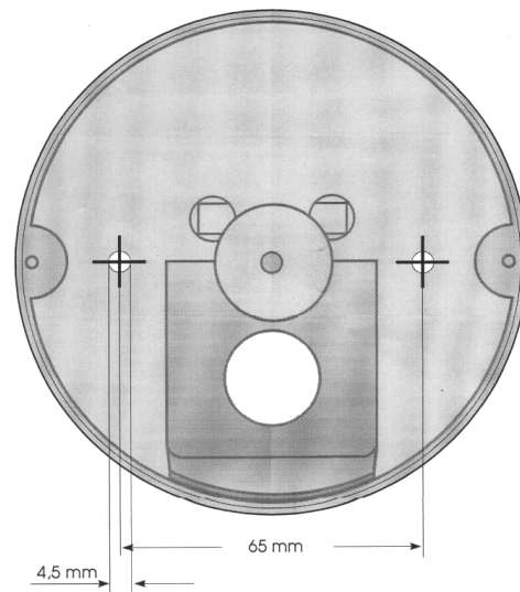
Fig.5: mounting of the bottom part
