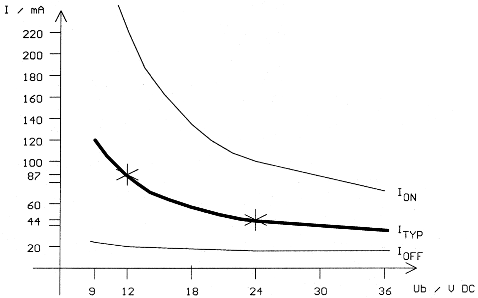
Fig.3: current vs. input voltage
