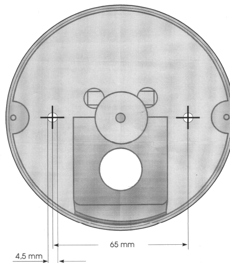
mounting drills at the bottom part
